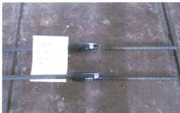
Figure 1 The failure occurred at the deformed bar when applied the maximum load.
