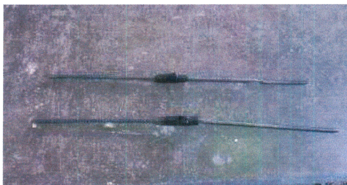
Figure 1 Tensile failure of deformed bar.
